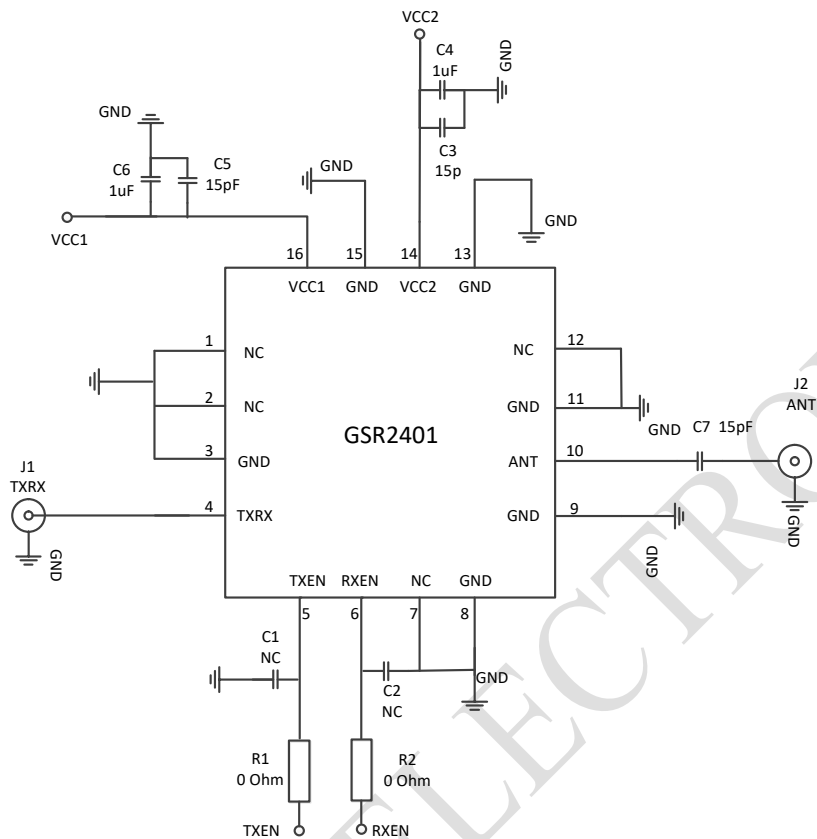
Figure 3 GSR2401 Application Schematic
