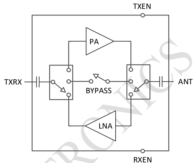
Figure 2 Block Diagram
